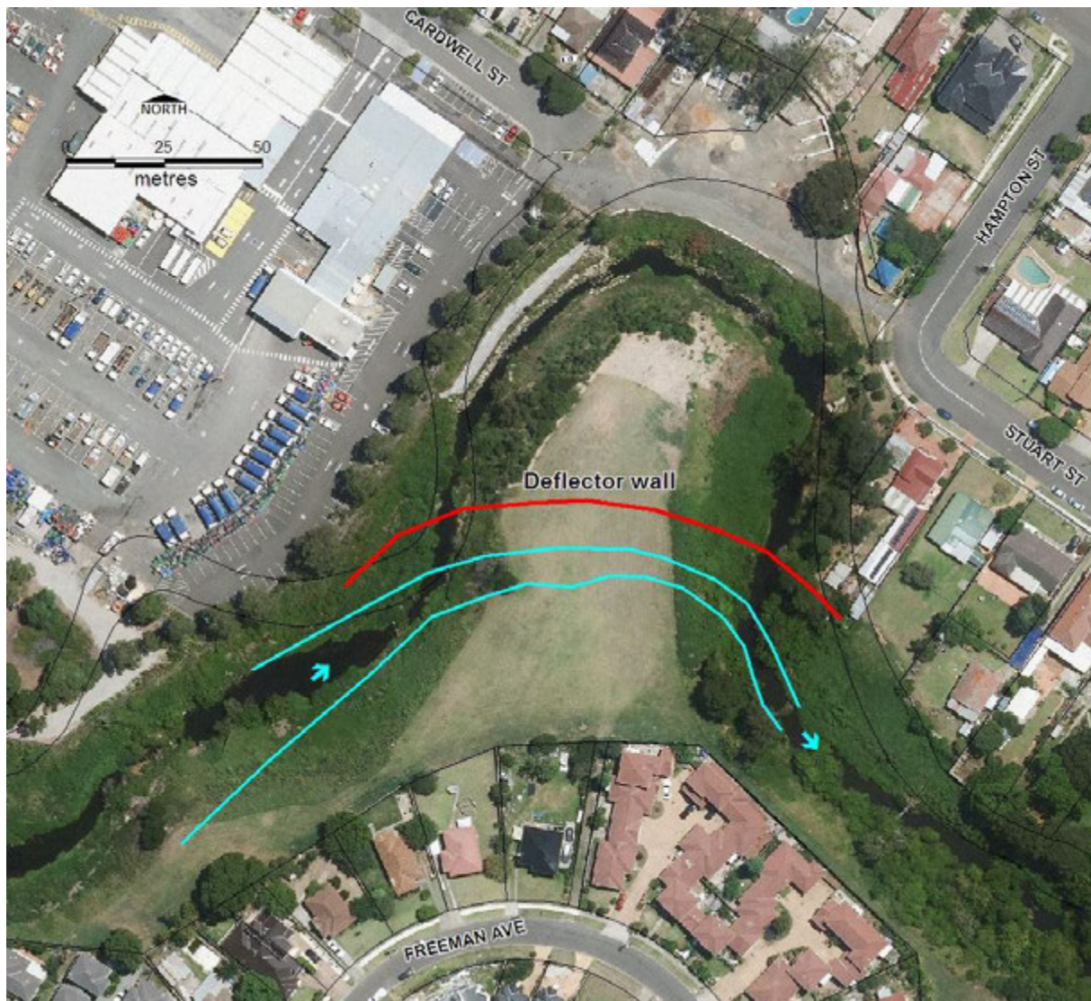
Figure 38 – Proposed channel realignment, Orphan School Creek near Freeman Avenue (after Dalland and Lucas, 1996)
