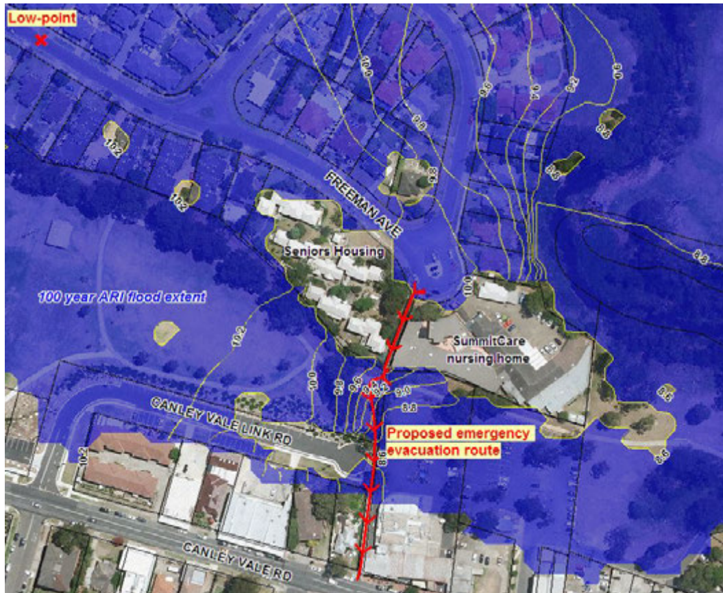
Figure 48 – Proposed Freeman Avenue emergency evacuation route
